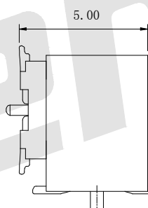
Mating Height:5.0mm
